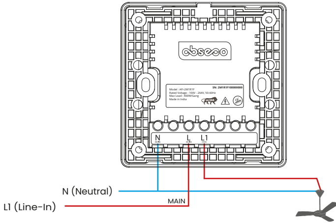
Figure : Wiring Diagram
